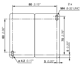
AF26, AF30, AF38 + VEM4 mechanical and electrical interlock set
