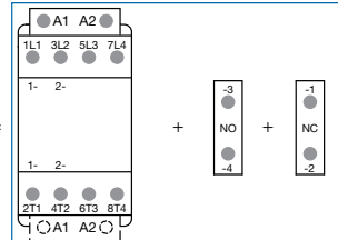
Combination 11 = AF09 ... AF38...-40-00 + CA4-10 + CA4-01
