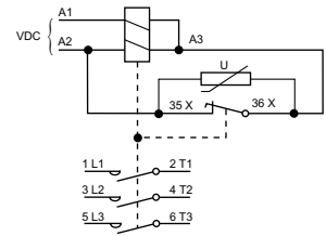
Coil wiring
