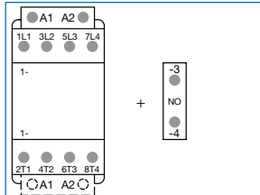
Combination 10 = AF09 ... AF38...-40-00 + CA4-10
