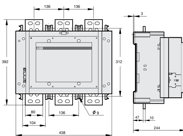
GAF1650, GAF2050 AF1350, AF1650, AF2050
