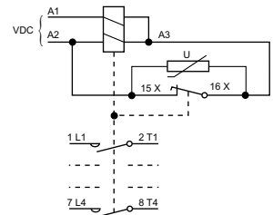
Coil wiring
