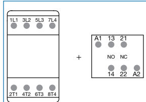
Combination 11 = AF09 ... AF38...-40-00 + CAT4-11E
