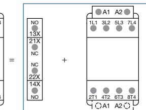
Combination 11 = CAL4-11 + AF09 ... AF38-40-00
