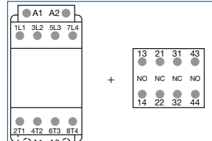
Combination 22 = AF09 ... AF38...-40-00 + CA4-22E
