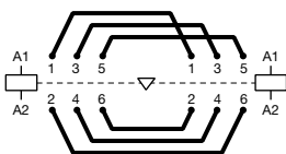
BER, BEM connection sets
